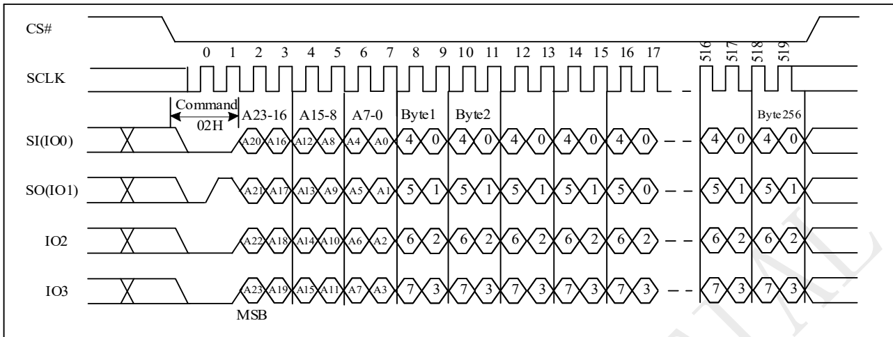
Figure 9-40a Page Program (PP) Sequence (QPI)
