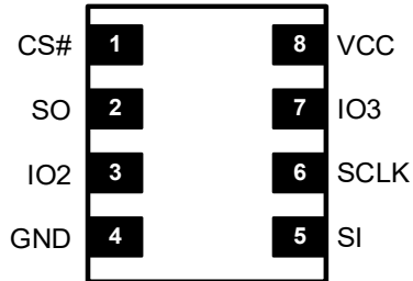
8-Pad WSON (8x6mm)
