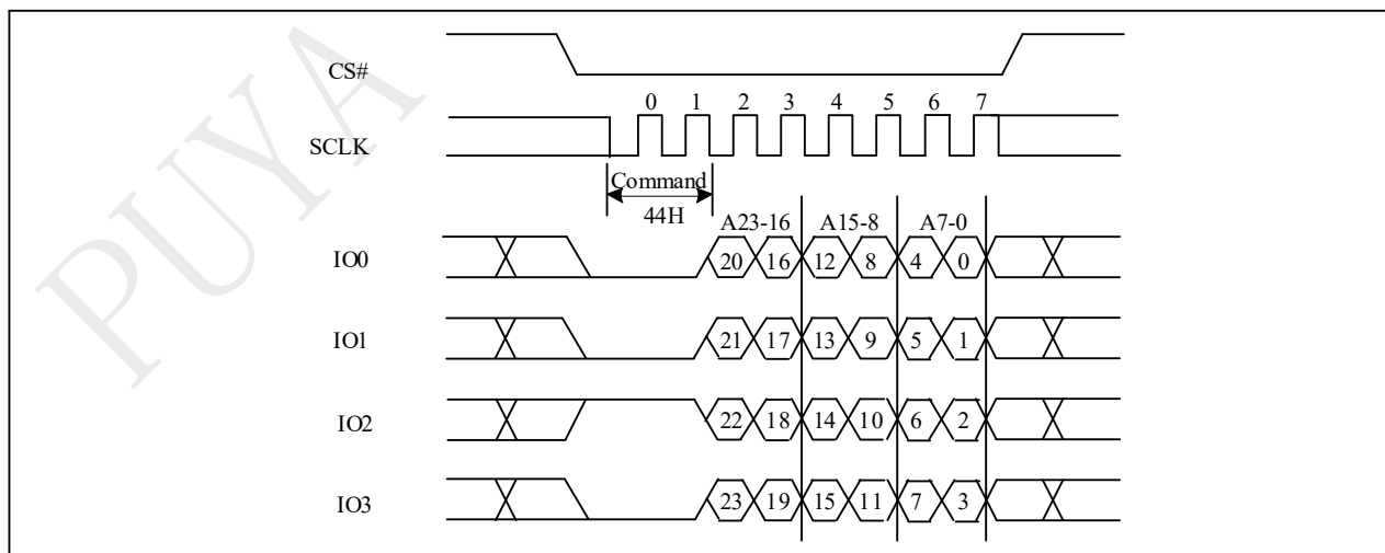
Figure 9-49a Erase Security Registers (ERSCUR) Sequence (QPI)
