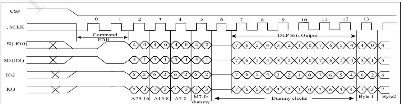
Figure 9-33k DTR 4IO Read with DLP bits output Sequence (QPI)
