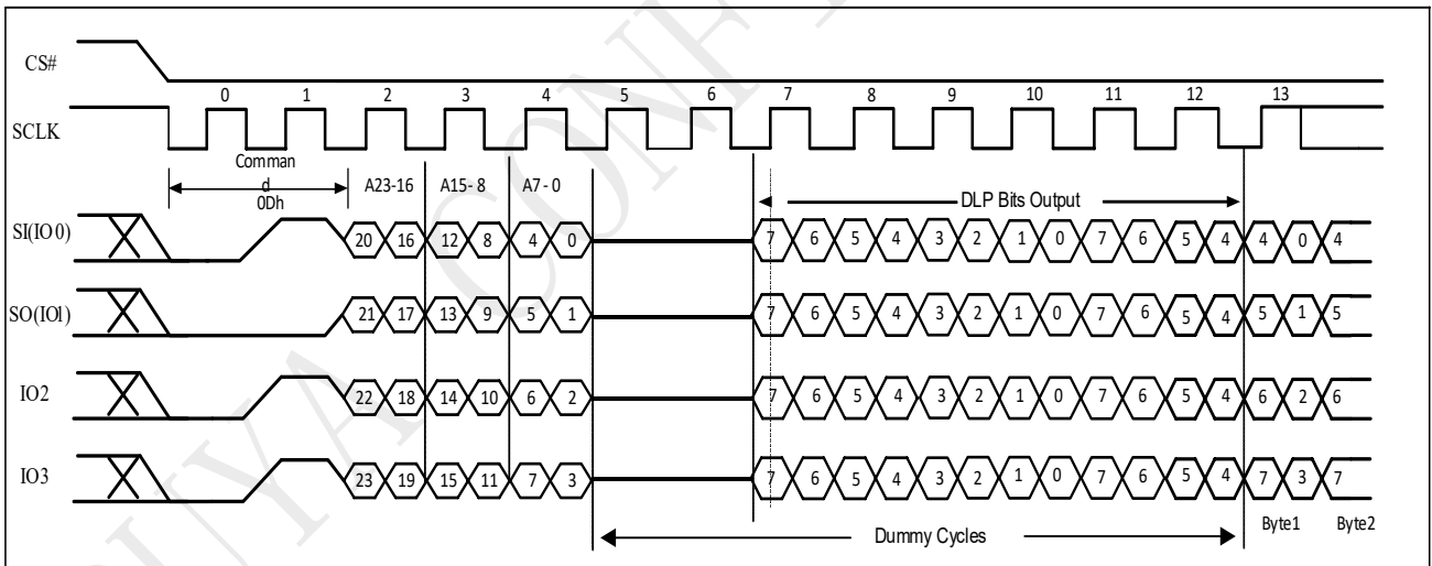
Figure 9-03h DTR 110 Read with DLP bits output Sequence (QPI)
